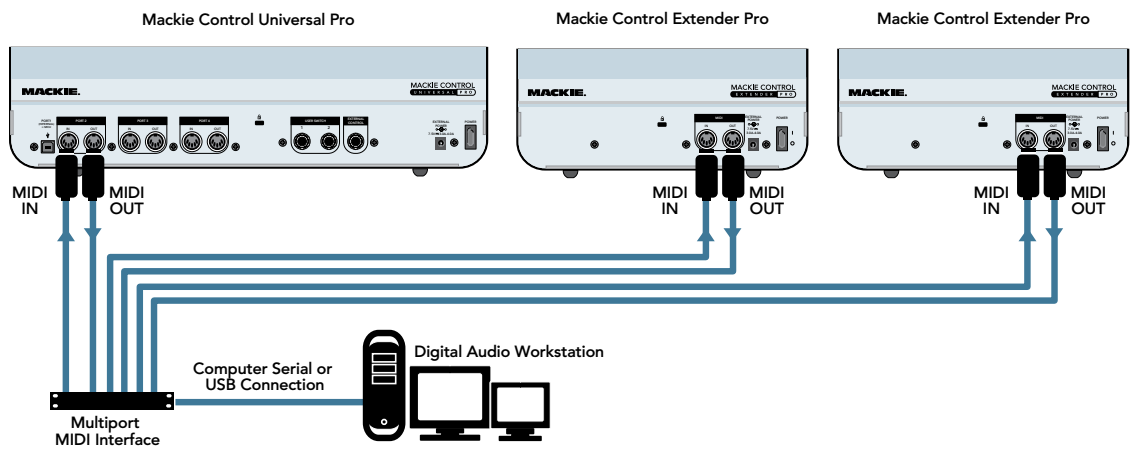
Hookup 2: MIDI
